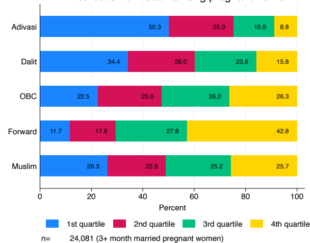
E. Distribution of wealth among pregnant women
